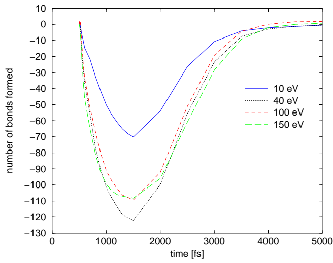
FIG. 1. The average bond destruction and annealing after a deposition event when the final position of the deposited atom is on the surface ( z > -2 \text{ \AA} i.e. surface-deposition). The deposition takes place at t = 500 \text{ fs} .
