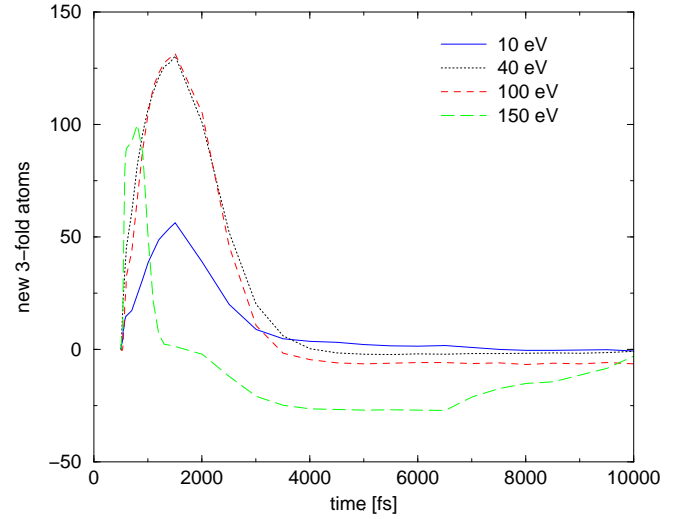
FIG. 4. The average formation of 3-fold coordinated atoms in the subsurface region. The deposition takes place at t = 500 \text{ fs} . The final position of the deposited atom is on the surface ( z > -2 \text{ \AA} i.e. surface-deposition).
