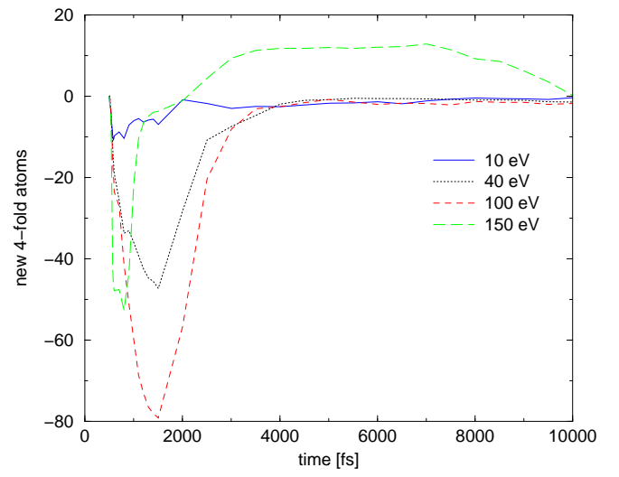
FIG. 3. The average formation of 4-fold coordinated atoms in the subsurface region. The deposition takes place at t = 500 \text{ fs} . The final position of the deposited atom is on the surface ( z > -2 \text{ \AA} i.e. surface-deposition).
