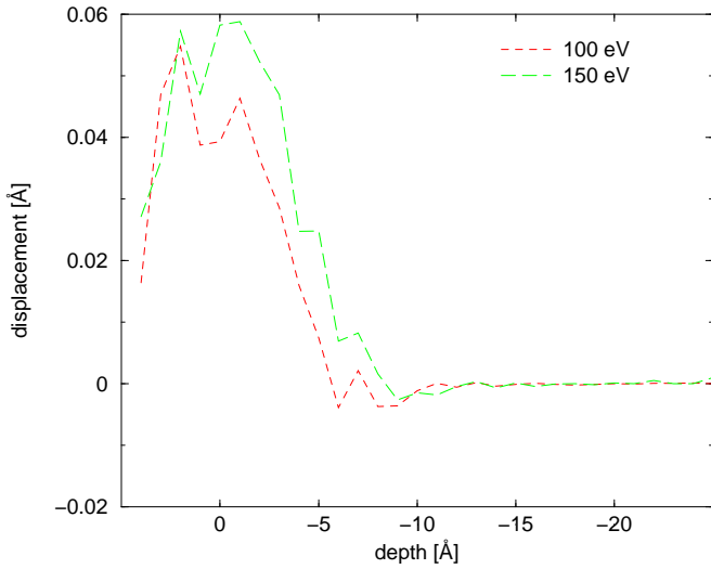
FIG. 2. The average displacements of the atoms in the growing film after a deposition event, when subplantation takes place ( z < -2 \text{ \AA} ). The instant surface position is at 0 \text{ \AA} .
