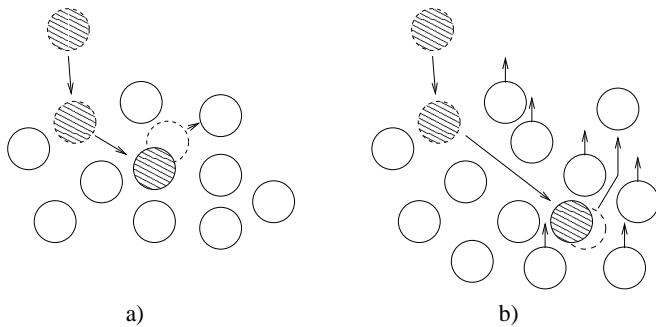
FIG. 6. a) At low energies the deposited atom may replace a former bulk atom. b) With higher energies subplantation may occur. The film grows by global expansion and individual atom diffusion. The deposited atom is a filled ball. The intermediate positions are dashed.
