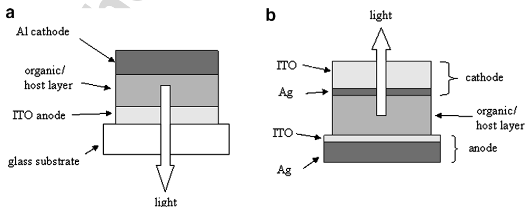
Fig. 1. Schematics of the (a) substrate-emitting and (b) top-emitting OLED structures investigated.
