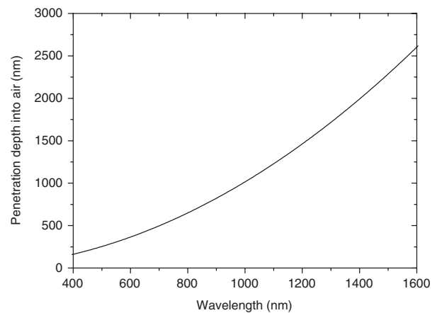
Figure 6. Showing how the penetration depth into the dielectric (here air) varies with free space wavelength in the visible and near-infrared. The data were computed using the Drude approximation for the relative permittivity of the metal (with \omega_p and \Gamma for silver taken to be \omega_p = 1.2 \times 10^{16} \text{ rad s}^{-1} ( \equiv 7.9 \text{ eV} ) and \Gamma = 1.45 \times 10^{13} \text{ s}^{-1} ( \equiv 0.06 \text{ eV} ) respectively). The relative permittivity of the dielectric was taken to be equal to 1.
