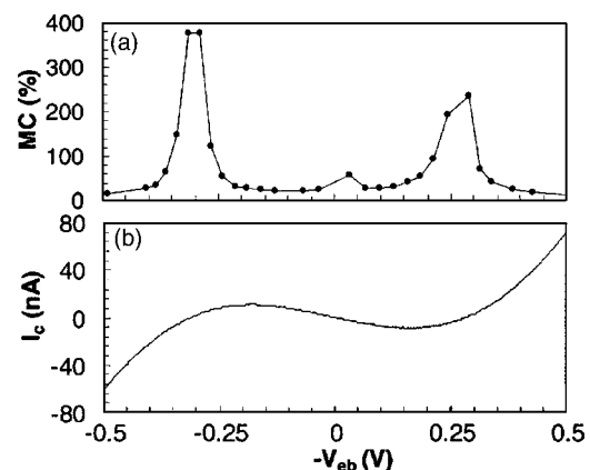
FIG. 5. (a) The bias dependence of the magnetocurrent obtained from a DBMTJ grown on a \text{Si}/\text{SiO}_2 substrate is shown (b) The corresponding I_c - V_{eb} characteristic is shown.
