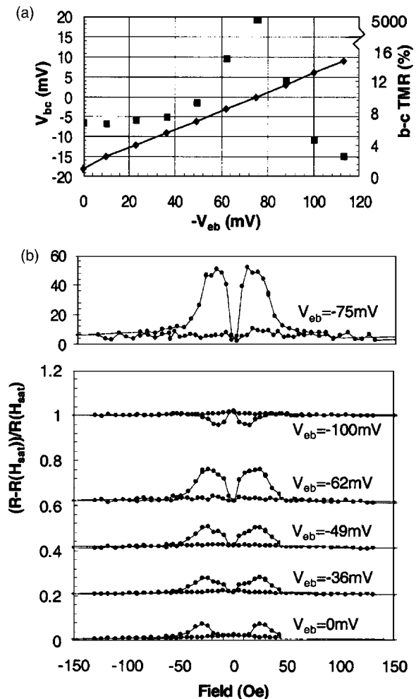
FIG. 4. (a) The dependence of the \text{Co}_b - \text{Co}_c junction TMR and the measured value of V_{bc} upon V_{eb} is shown for a DBMTJ grown upon a quartz substrate. A bias of 18 mV was applied to the b - c circuit. (b) The shape of the \text{Co}_b - \text{Co}_c TMR characteristic at \theta=50^\circ is shown for different values of V_{eb} . The lower 6 curves have been offset for clarity.
