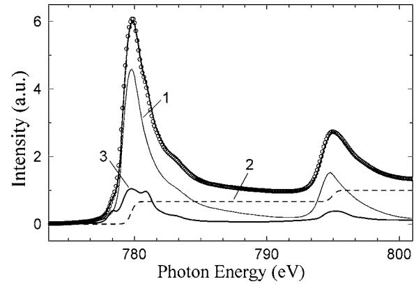
FIG. 2. Magnetization-averaged x-ray absorption spectrum measured from the 360 s barrier oxidation sample (open circles) and best-fit model (solid line), using a superposition of the curves labeled 1–3.
