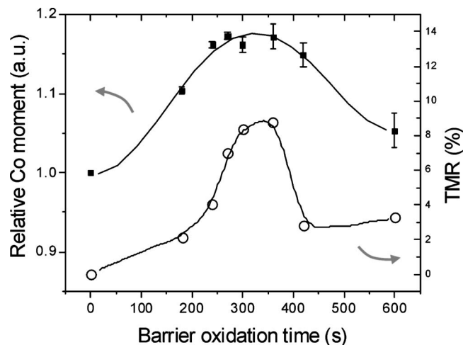
FIG. 3. Relative Co moment determined by XMCD as a function of barrier oxidation time following the fitting and normalization procedure. The measured TMR values are also given. Drawn lines are guides to the eye.
