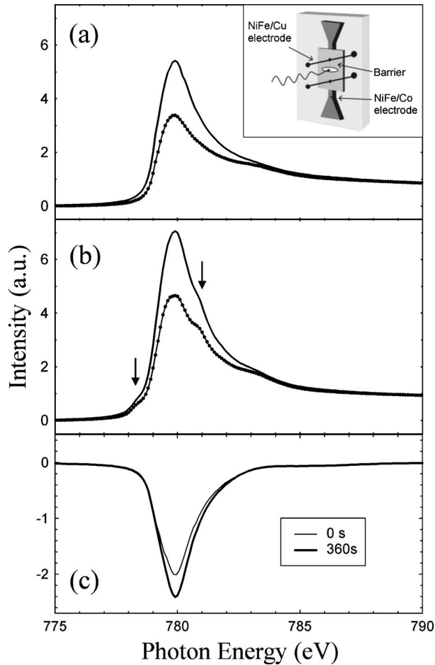
FIG. 1. X-ray absorption spectra measured across the Co L_3 absorption edge for the two saturation magnetization directions (symbols and solid lines), for barrier oxidation times of: (a) 0 s and (b) 360 s. The difference spectra (XMCD) for the 0 s and 360 s sample are shown in (c). The inset shows the sample geometry used.
