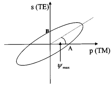
FIG. 1. A schematic of the ellipse describing the light reflected from a Kretschmann SP system with incident light consisting of both s and p components. \psi_{\max} is the azimuth of the ellipse, with A and B being the purely p and s components.
